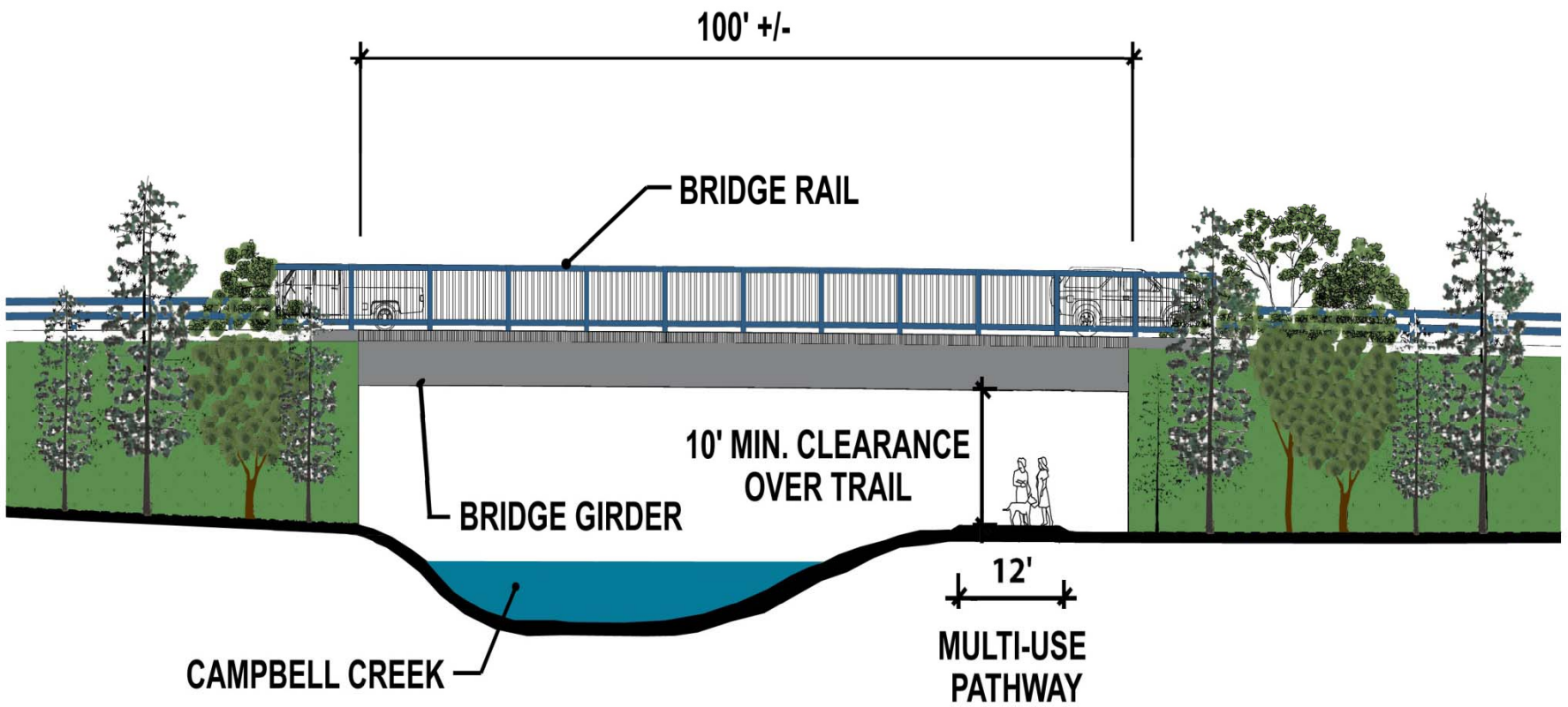
BRIDGE SIDE VIEW SECTION CAMPBELL CREEK BRIDGE
