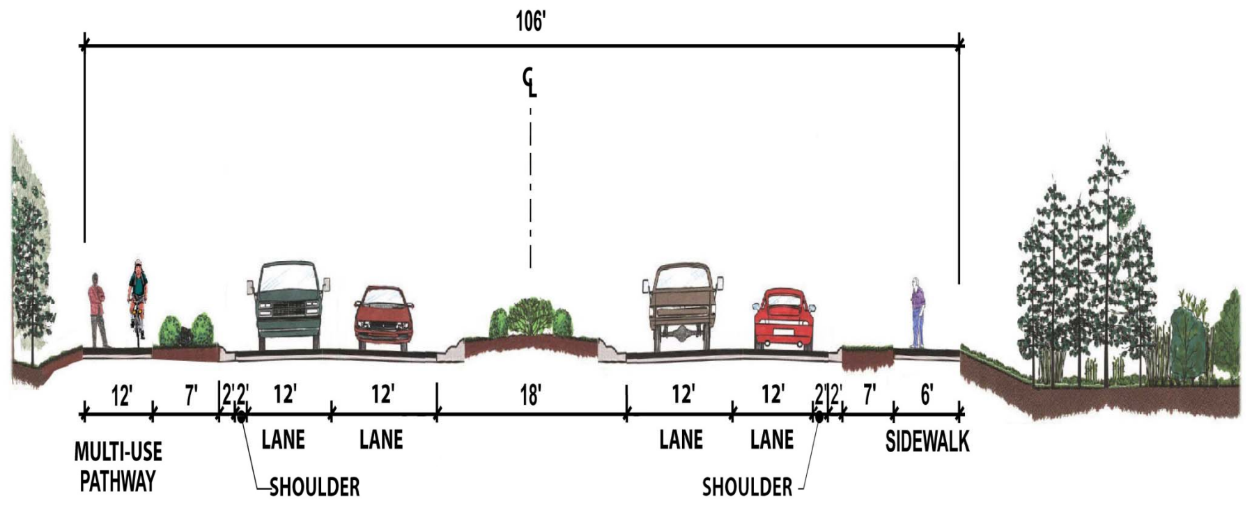
URBAN TYPICAL SECTION C STREET TO OLD SEWARD HIGHWAY TYPICAL SECTION
