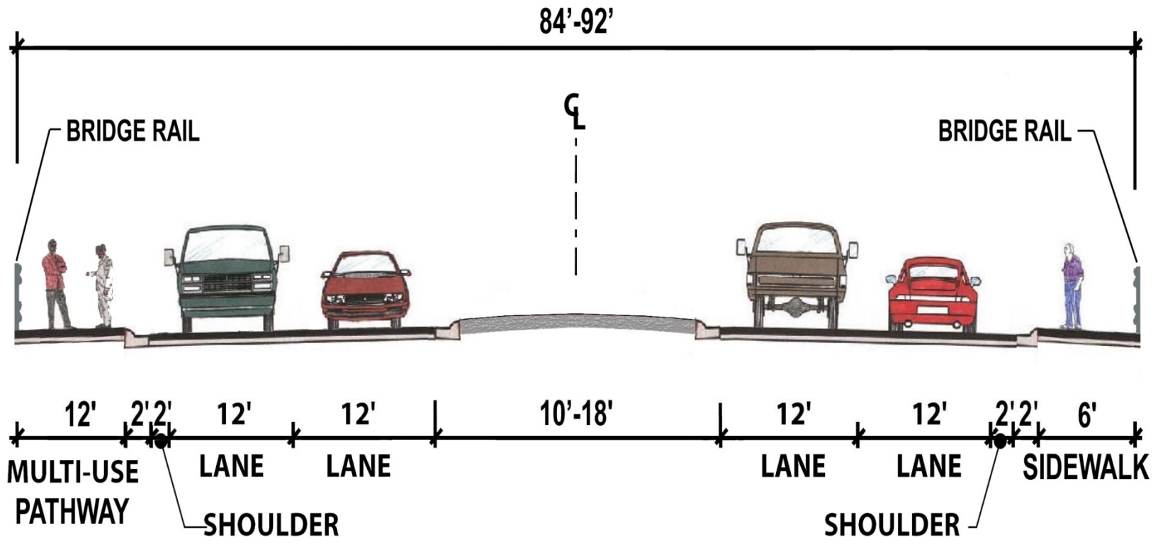
TYPICAL SECTION CAMPBELL CREEK BRIDGE
